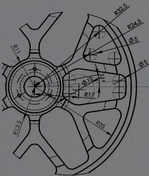
Detail E
